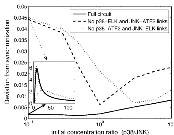
FIGURE 6 Deviation from synchronization of bifan motif and nonbifan circuits for a range of initial conditions. Deviation from synchronization was calculated as the root mean-square of the difference between normalized concentrations (see text for details). The network is the same as in Fig. 5 and the initial conditions are: [ATF2] = [ELK] = 20 \mu M, [c-Jun] = 10 \mu M, [p38] = 3 \mu M, and [JNK] was varying from 0.3 to 30 \mu M. As an example, time course of free ATF2* and ELK* is presented in the inset for the case p38:JNK = 1:10. In the full bifan configuration (solid lines) the two lines coincide, whereas without the cross links (dotted line) the two TFs are not synchronized.
