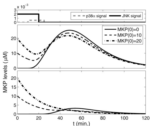
FIGURE 11 Effect of initial condition of MKP1 levels on the feedback loop dynamics. When the bifan synchronizes the dynamics of the transcription factors, the feedback loop is highly active (upper panel). However, after eliminating the links from p38 to ELK1 and from JNK1 to ATF2 there is no more synchronization, and thus no transcription of MKP1 observed (lower panel).
