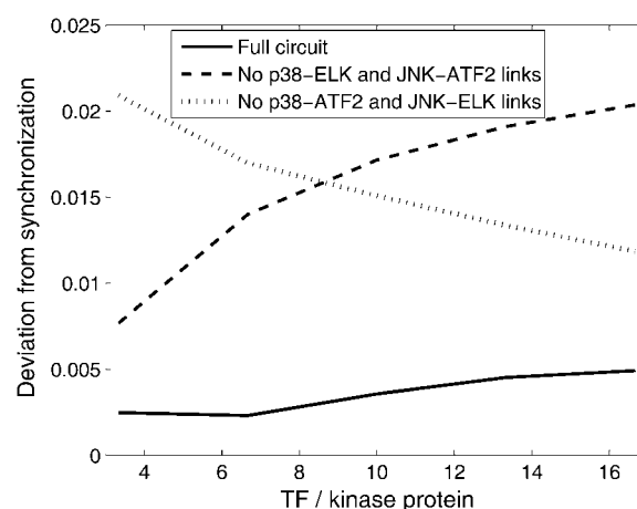
FIGURE 7 Deviation from synchronization of bifan motif and nonbifan circuits for a range of initial conditions. The network is the same as in Fig. 5. The initial conditions are: [p38] = [JNK] = 3 \mu M, [ATF2], [ELK], and [c-Jun] varying between 10 \mu M to 50 \mu M, yielding TF/kinase ratios between 3 and 17.
